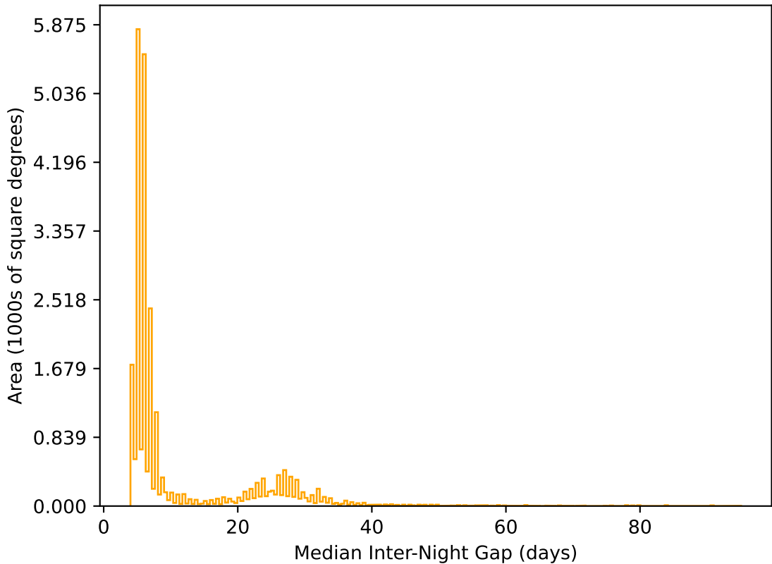
ddf_loaded_half_fl2_v3.4_10yrs All sky r band: Median Inter-Night Gap
