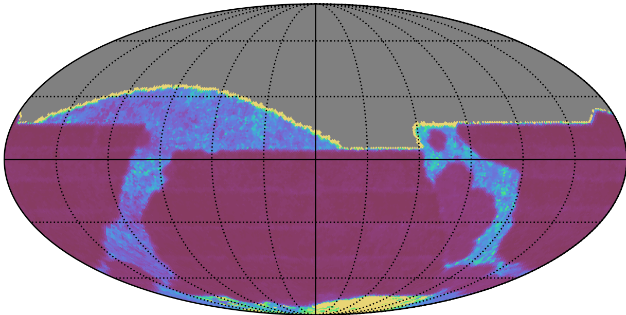
ddf_loaded_half_fl2_v3.4_10yrs All sky i band: Median Inter-Night Gap
