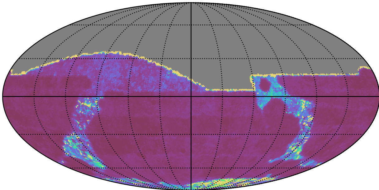
ddf_loaded_half_fl2_v3.4_10yrs All sky g band: Median Inter-Night Gap
