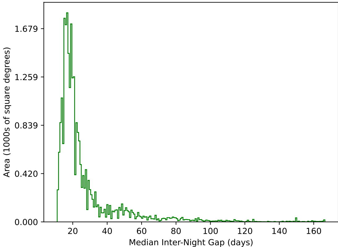
ddf_loaded_half_fl2_v3.4_10yrs All sky g band: Median Inter-Night Gap
