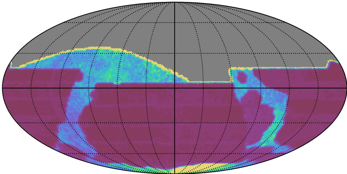
ddf_loaded_half_fl2_v3.4_10yrs All sky all bands: Median Inter-Night Gap
