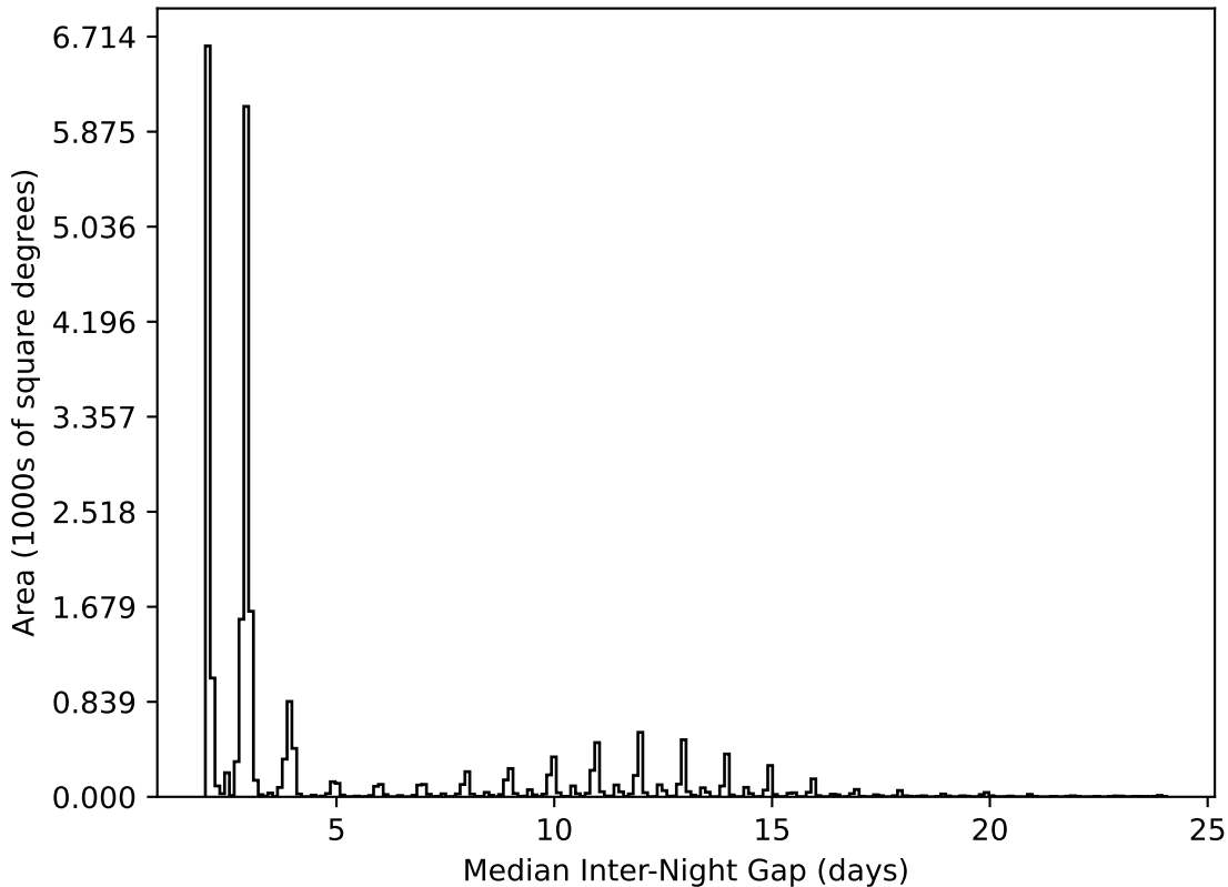
ddf_loaded_half_fl2_v3.4_10yrs All sky all bands: Median Inter-Night Gap
