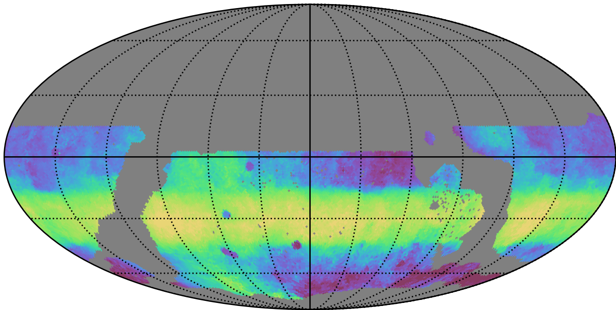
ddf_loaded_half_fl2_v3.4_10yrs WFD z band: Median HA
