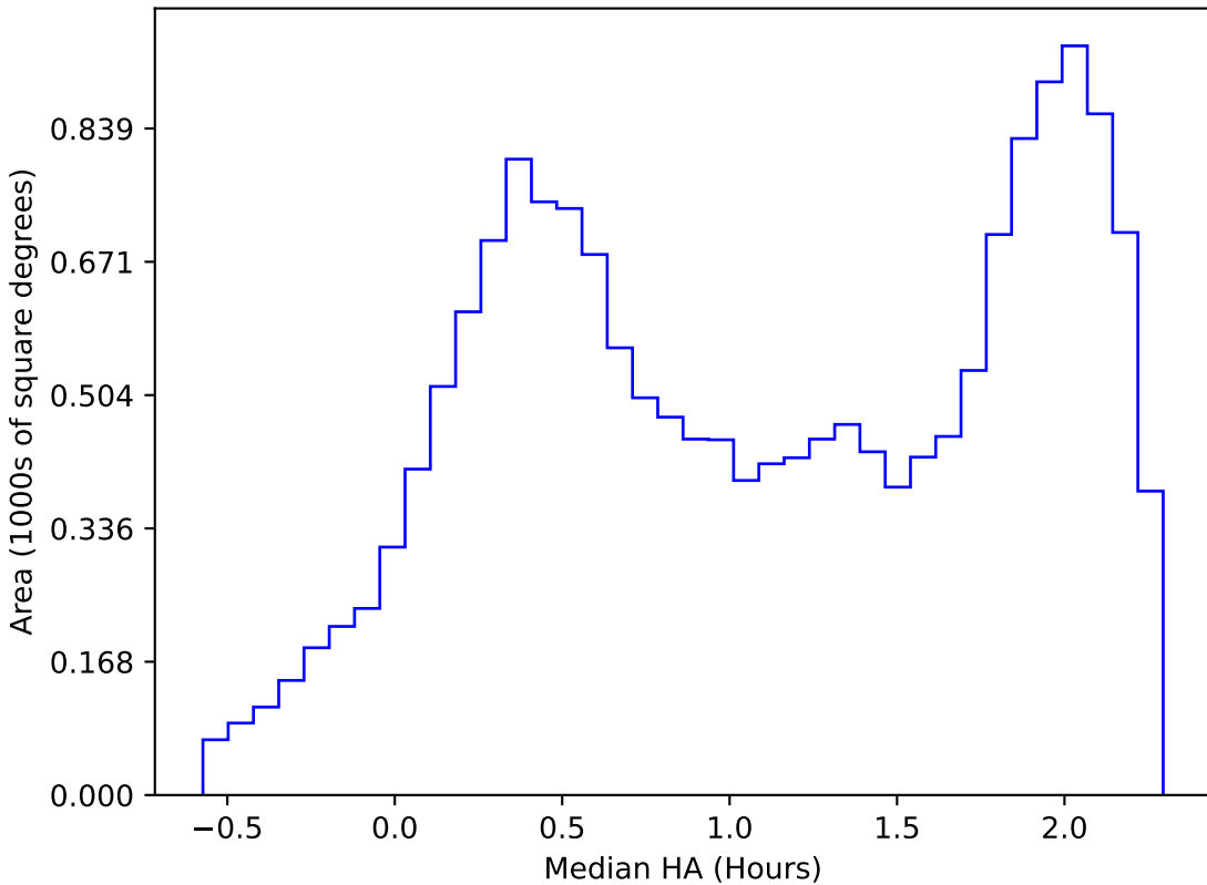
ddf_loaded_half_fl2_v3.4_10yrs WFD z band: Median HA
