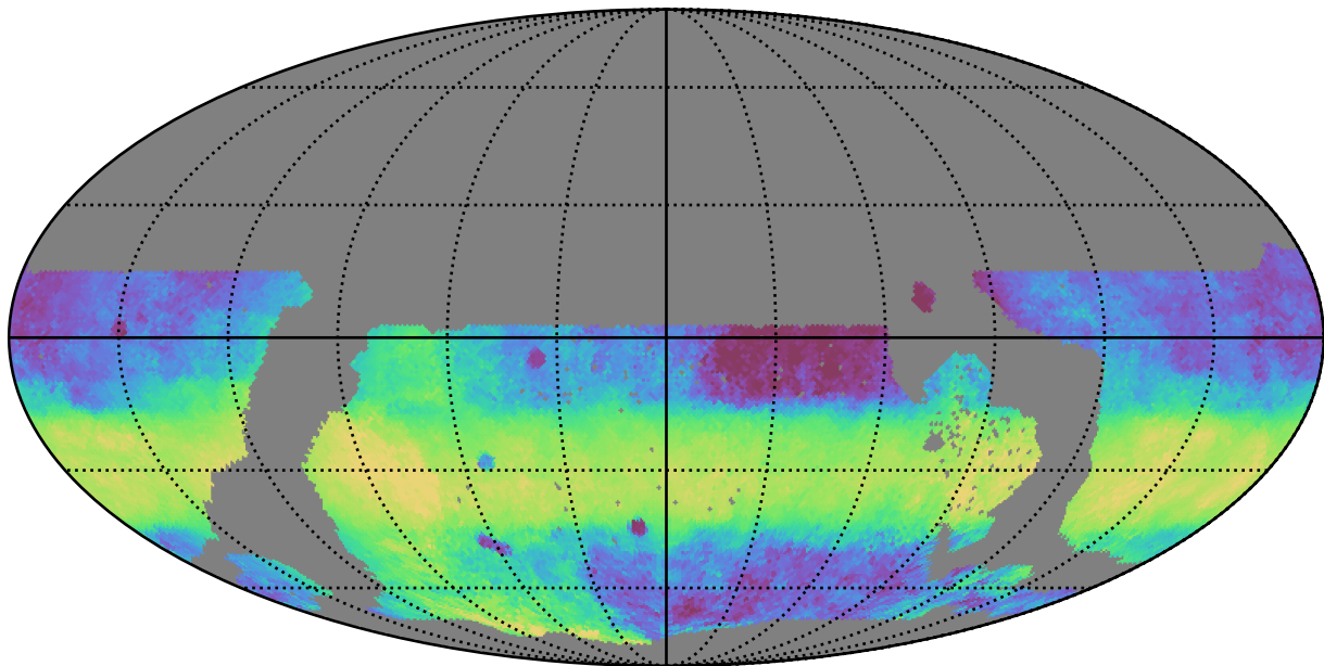
ddf_loaded_half_fl2_v3.4_10yrs WFD y band: Median HA
