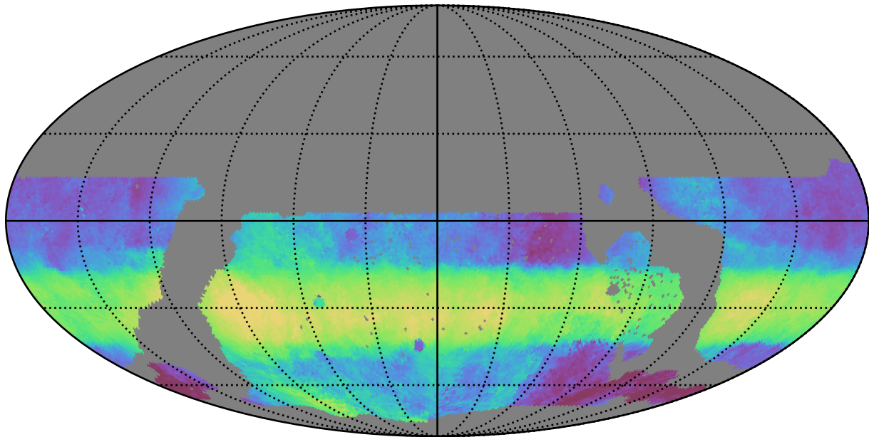
ddf_loaded_half_fl2_v3.4_10yrs WFD r band: Median HA
