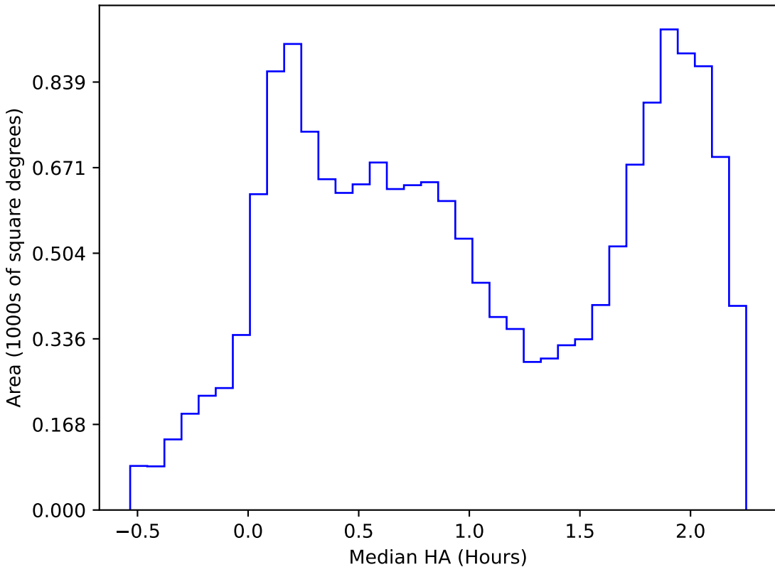
ddf_loaded_half_fl2_v3.4_10yrs WFD i band: Median HA
