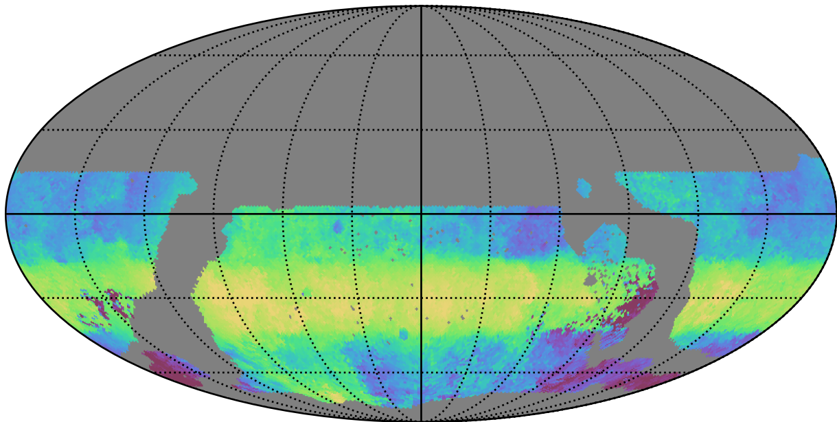
ddf_loaded_half_fl2_v3.4_10yrs WFD g band: Median HA
