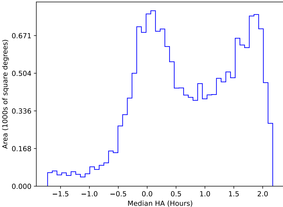
ddf_loaded_half_fl2_v3.4_10yrs WFD g band: Median HA
