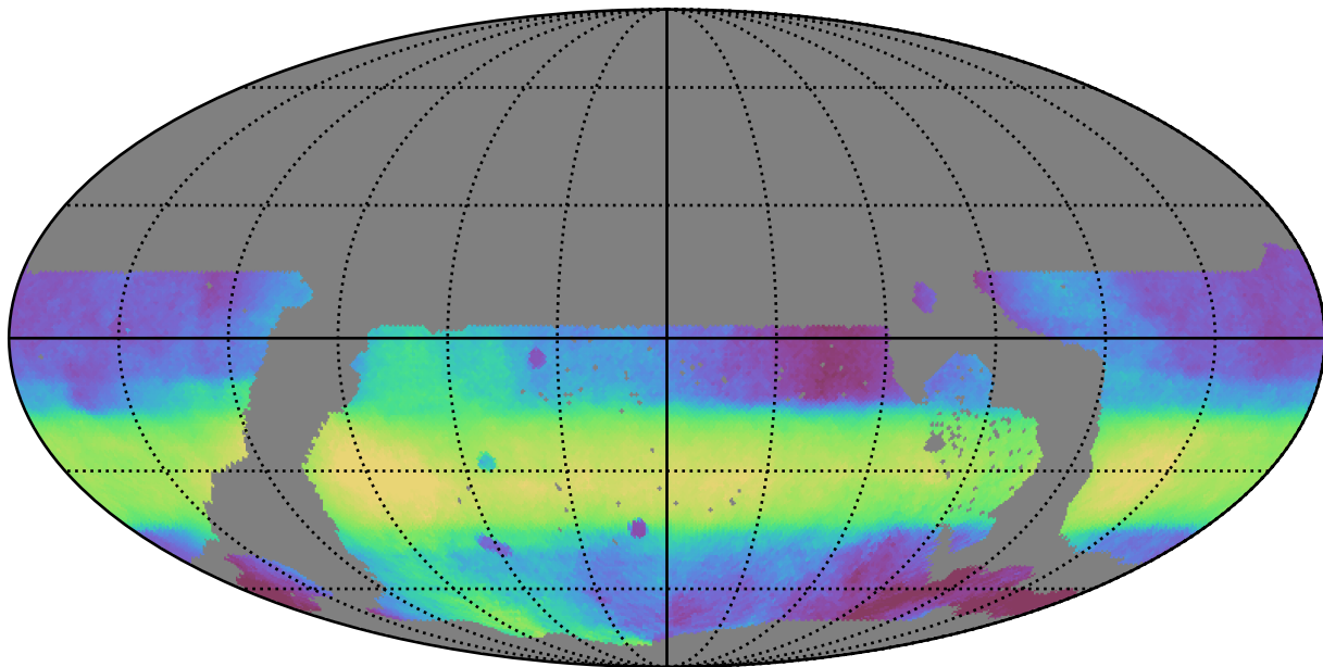
ddf_loaded_half_fl2_v3.4_10yrs WFD all bands: Median HA
