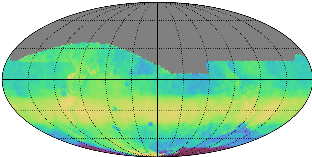
ddf_loaded_half_fl2_v3.4_10yrs All sky z band: Median HA
