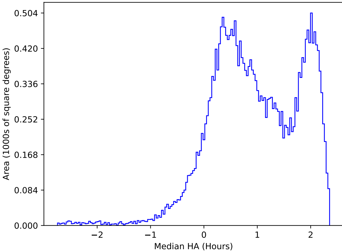
ddf_loaded_half_fl2_v3.4_10yrs All sky z band: Median HA
