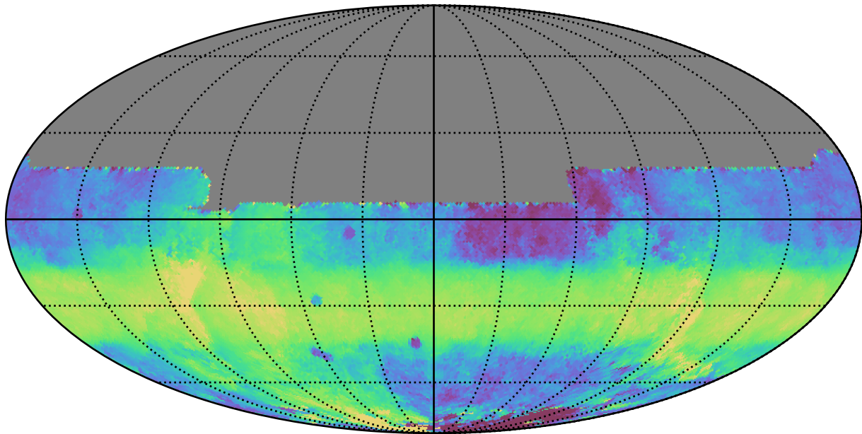
ddf_loaded_half_f12_v3.4_10yrs All sky y band: Median HA
