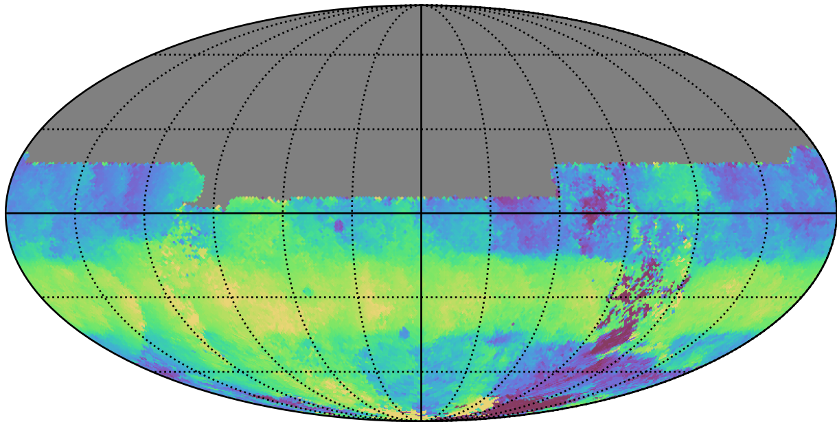
ddf_loaded_half_fl2_v3.4_10yrs All sky u band: Median HA
