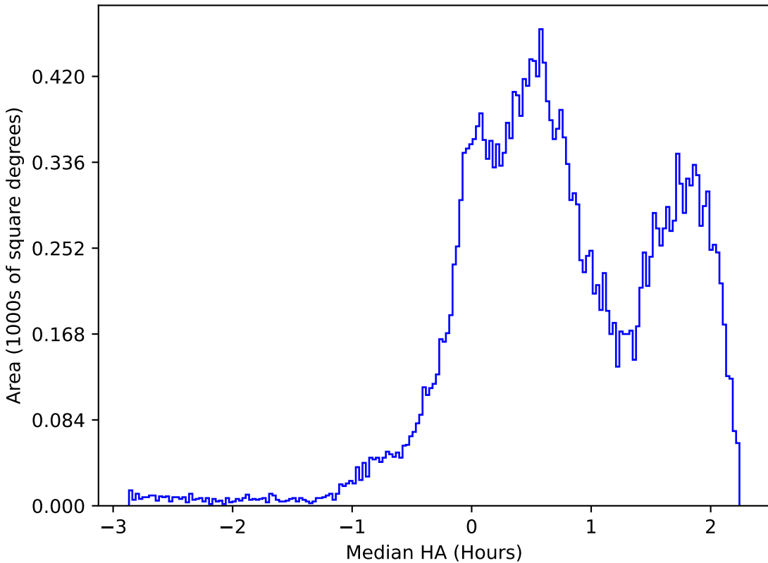
ddf_loaded_half_fl2_v3.4_10yrs All sky r band: Median HA
