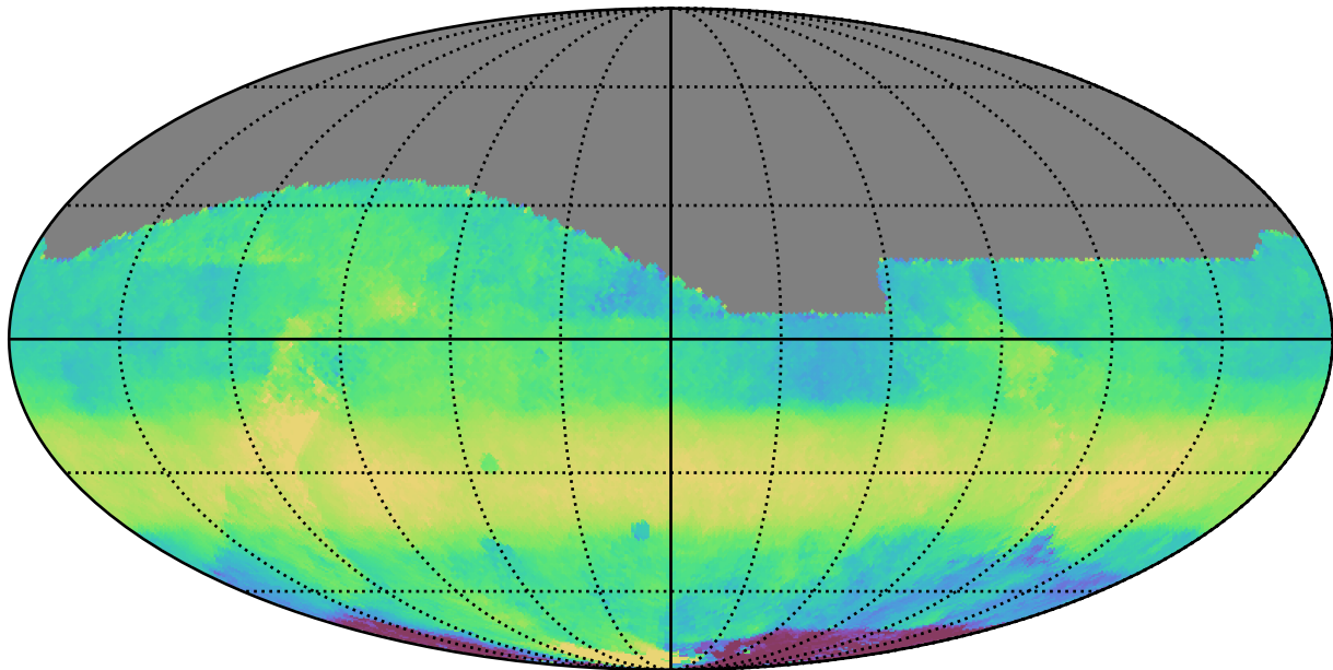
ddf_loaded_half_fl2_v3.4_10yrs All sky i band: Median HA
