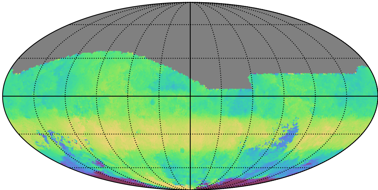
ddf_loaded_half_fl2_v3.4_10yrs All sky g band: Median HA
