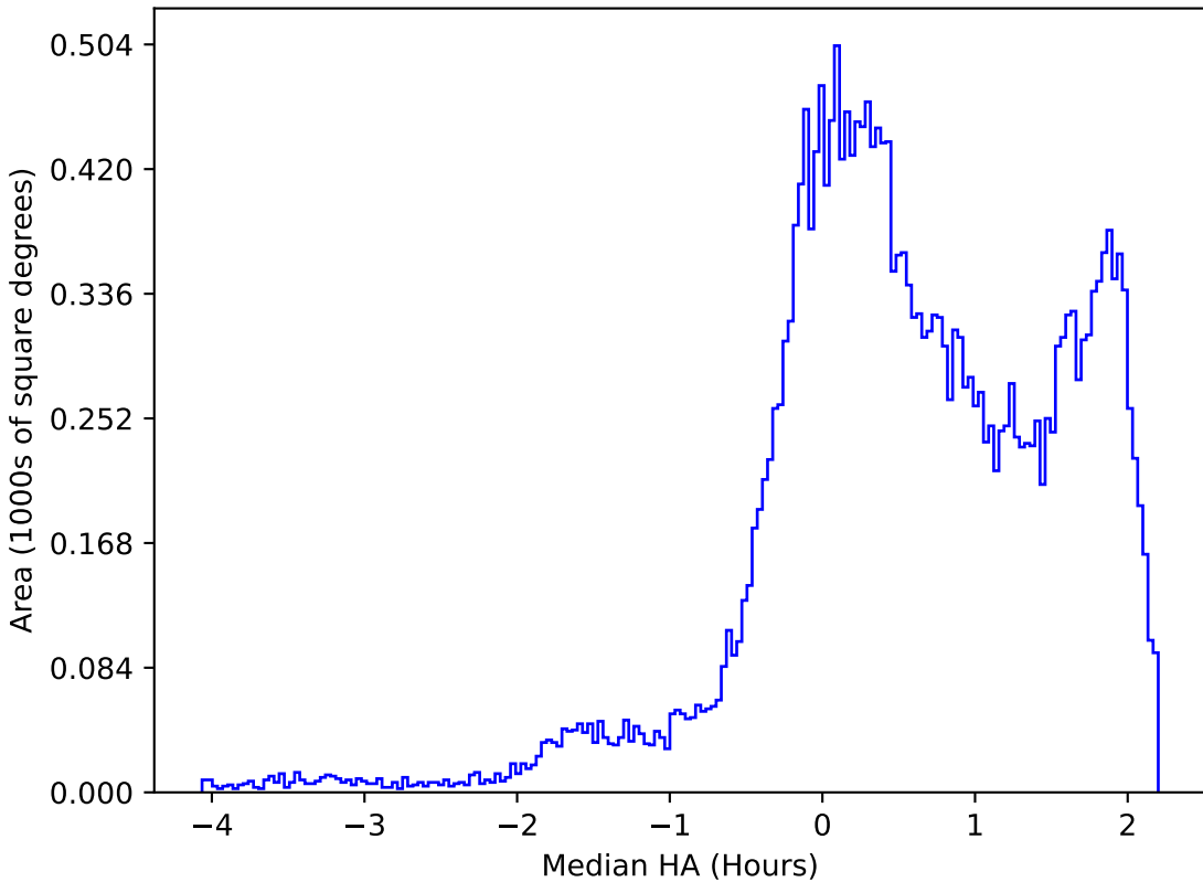
ddf_loaded_half_fl2_v3.4_10yrs All sky g band: Median HA
