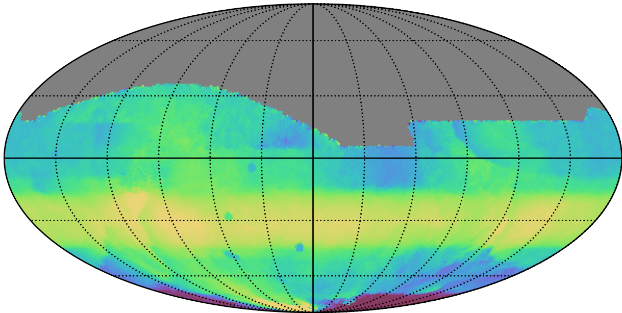
ddf_loaded_half_fl2_v3.4_10yrs All sky all bands: Median HA
