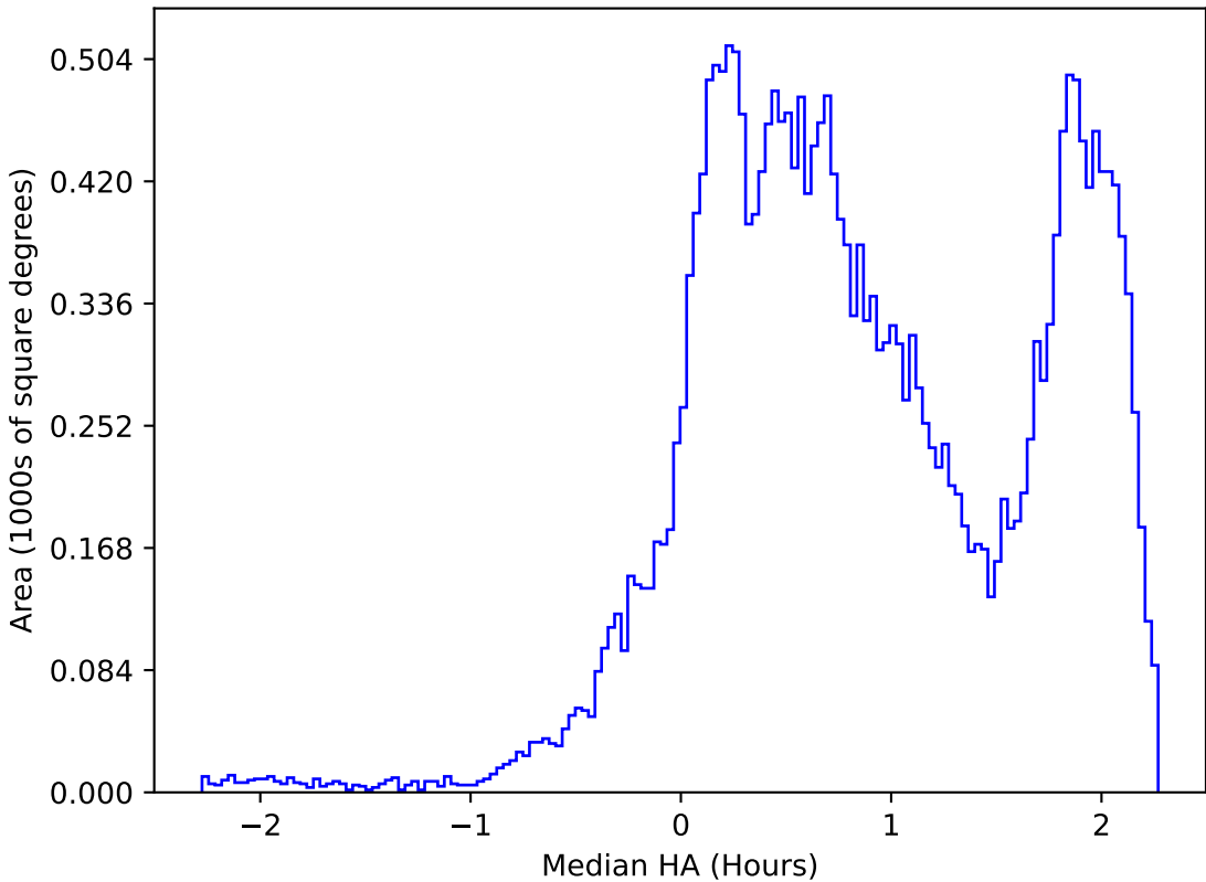
ddf_loaded_half_fl2_v3.4_10yrs All sky all bands: Median HA
