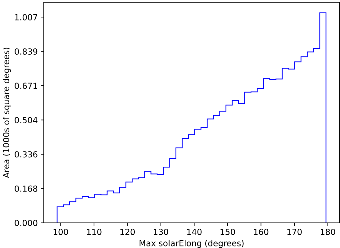
ddf_loaded_half_fl2_v3.4_10yrs WFD z band: Max solarElong
