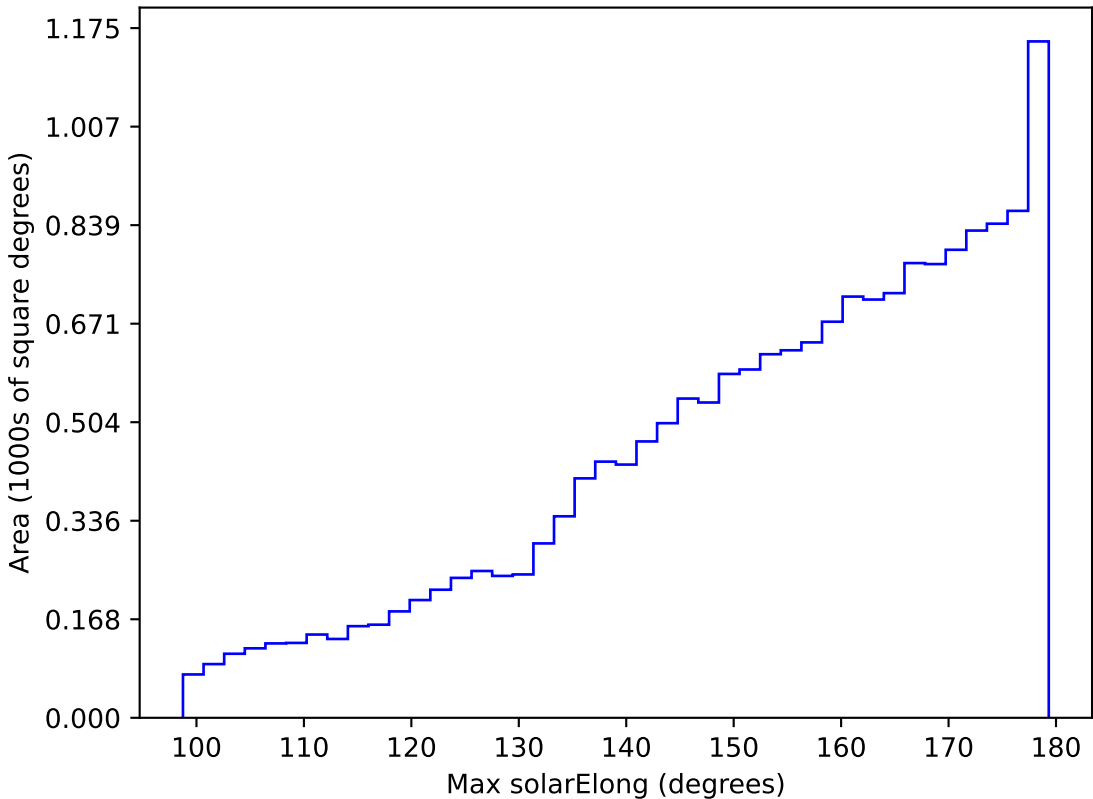
ddf_loaded_half_fl2_v3.4_10yrs WFD r band: Max solarElong
