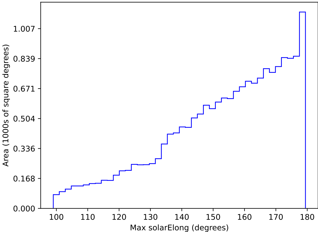
ddf_loaded_half_fl2_v3.4_10yrs WFD i band: Max solarElong
