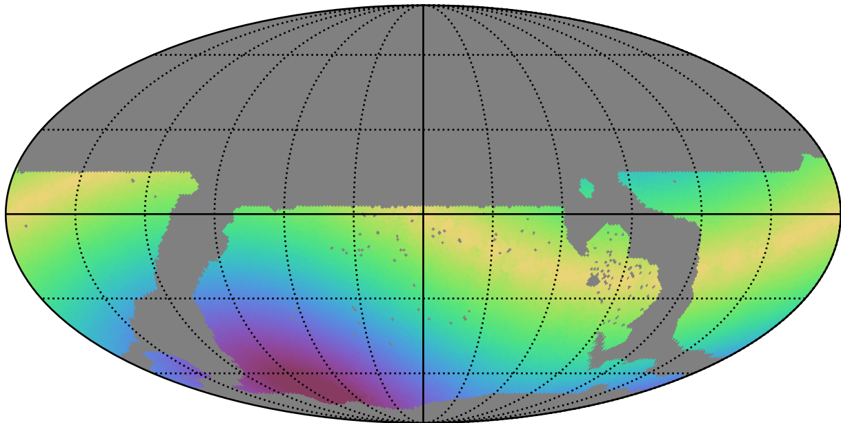
ddf_loaded_half_fl2_v3.4_10yrs WFD g band: Max solarElong
