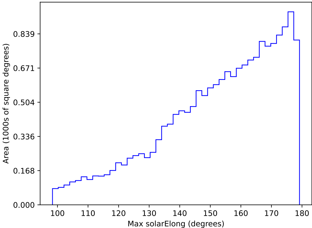
ddf_loaded_half_fl2_v3.4_10yrs WFD g band: Max solarElong
