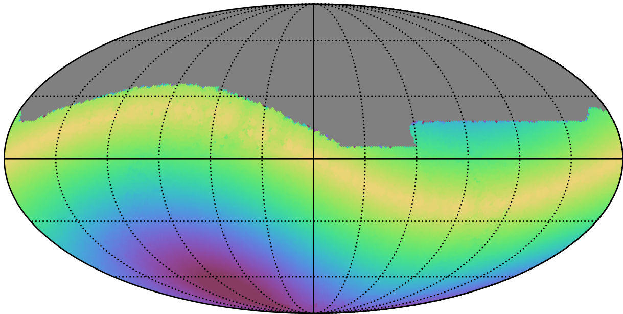
ddf_loaded_half_fl2_v3.4_10yrs All sky z band: Max solarElong
