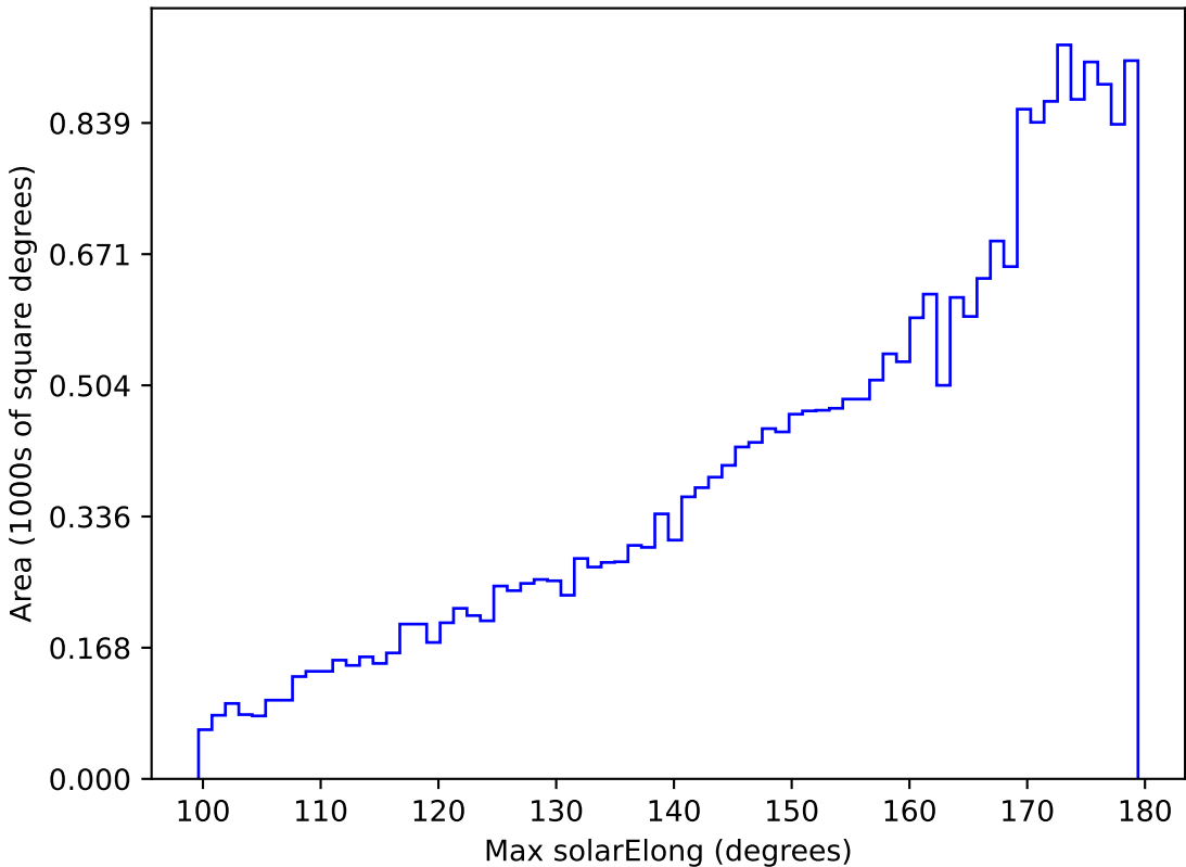
ddf_loaded_half_fl2_v3.4_10yrs All sky z band: Max solarElong
