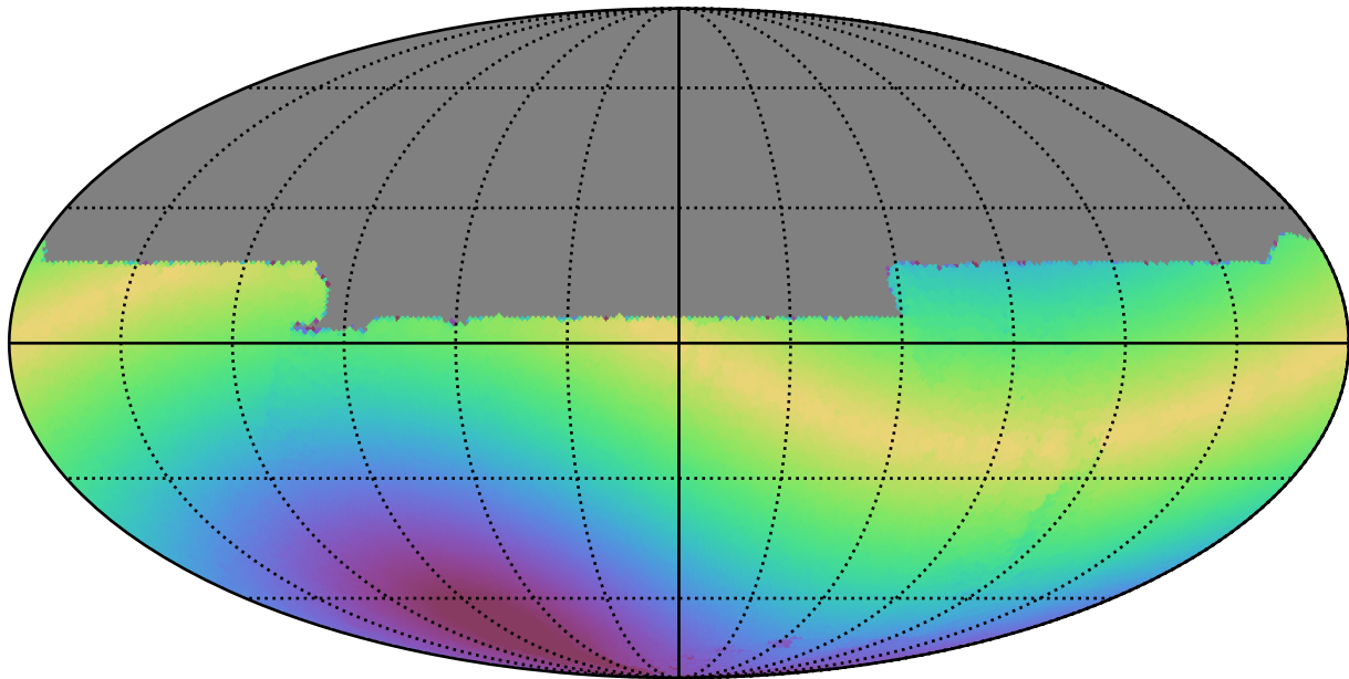
ddf_loaded_half_fl2_v3.4_10yrs All sky y band: Max solarElong
