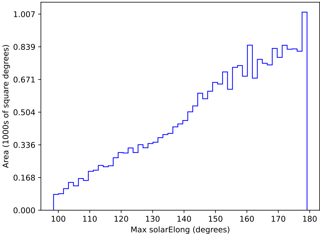
ddf_loaded_half_f12_v3.4_10yrs All sky y band: Max solarElong
