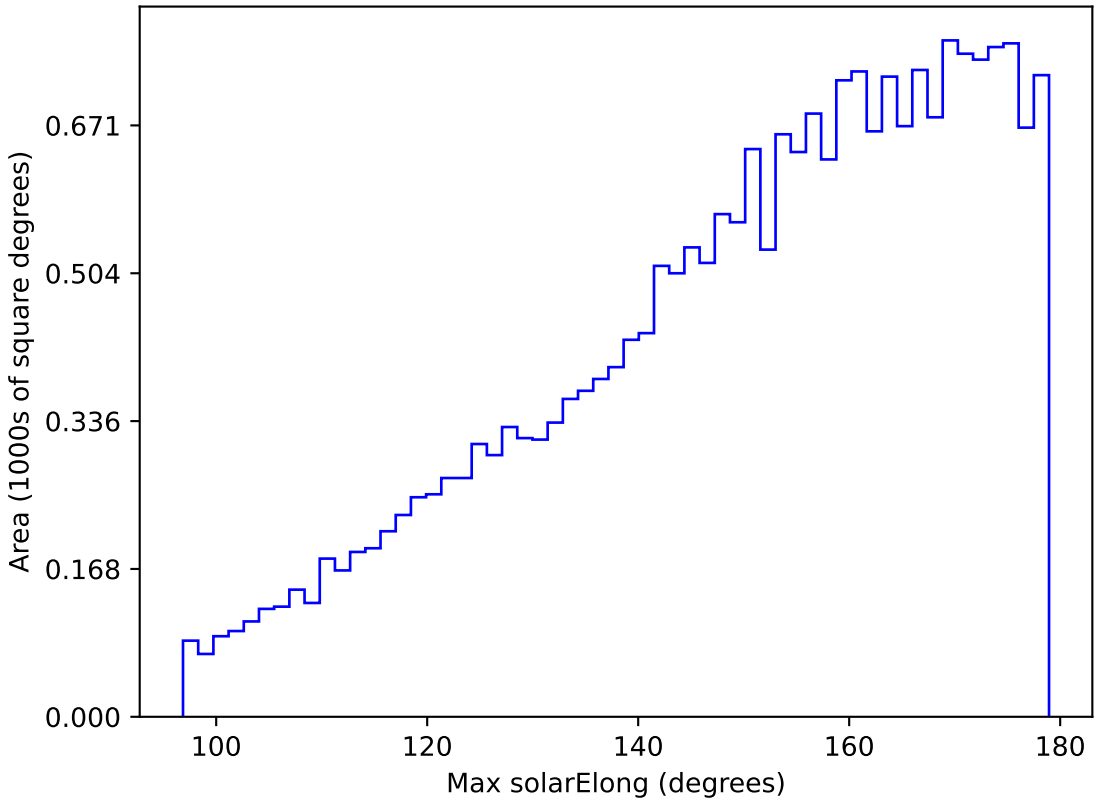
ddf_loaded_half_fl2_v3.4_10yrs All sky u band: Max solarElong
