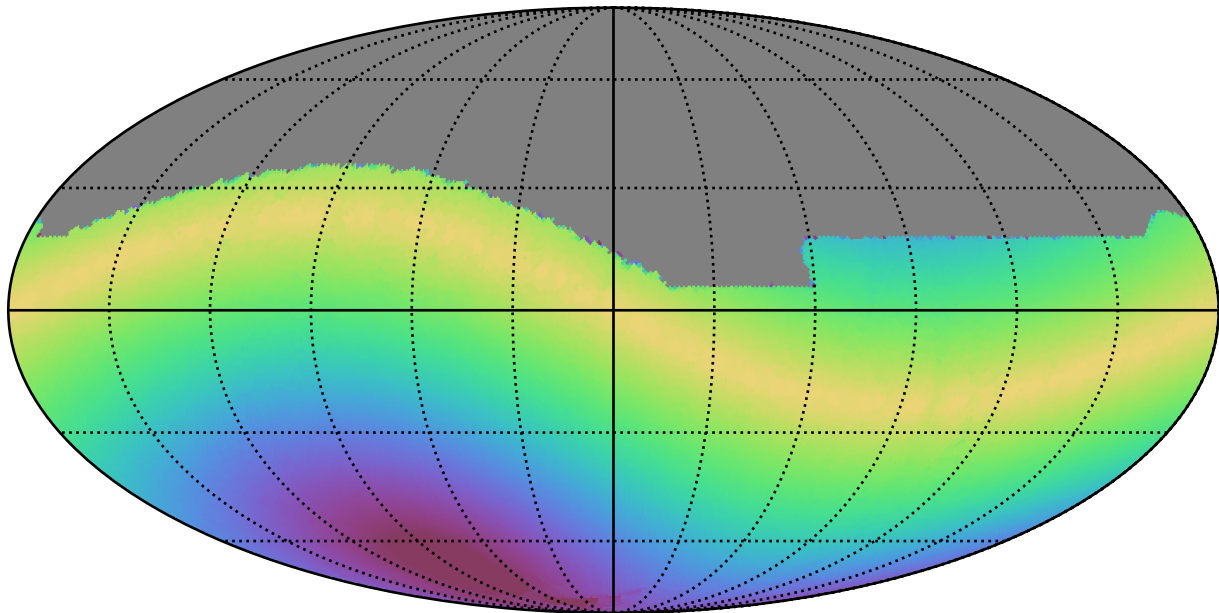
ddf_loaded_half_fl2_v3.4_10yrs All sky r band: Max solarElong
