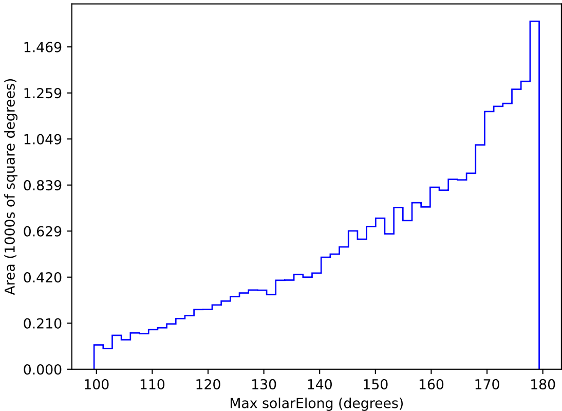
ddf_loaded_half_fl2_v3.4_10yrs All sky r band: Max solarElong
