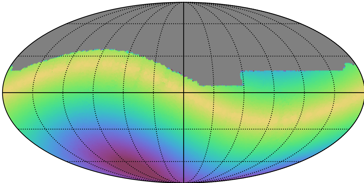
ddf_loaded_half_fl2_v3.4_10yrs All sky i band: Max solarElong
