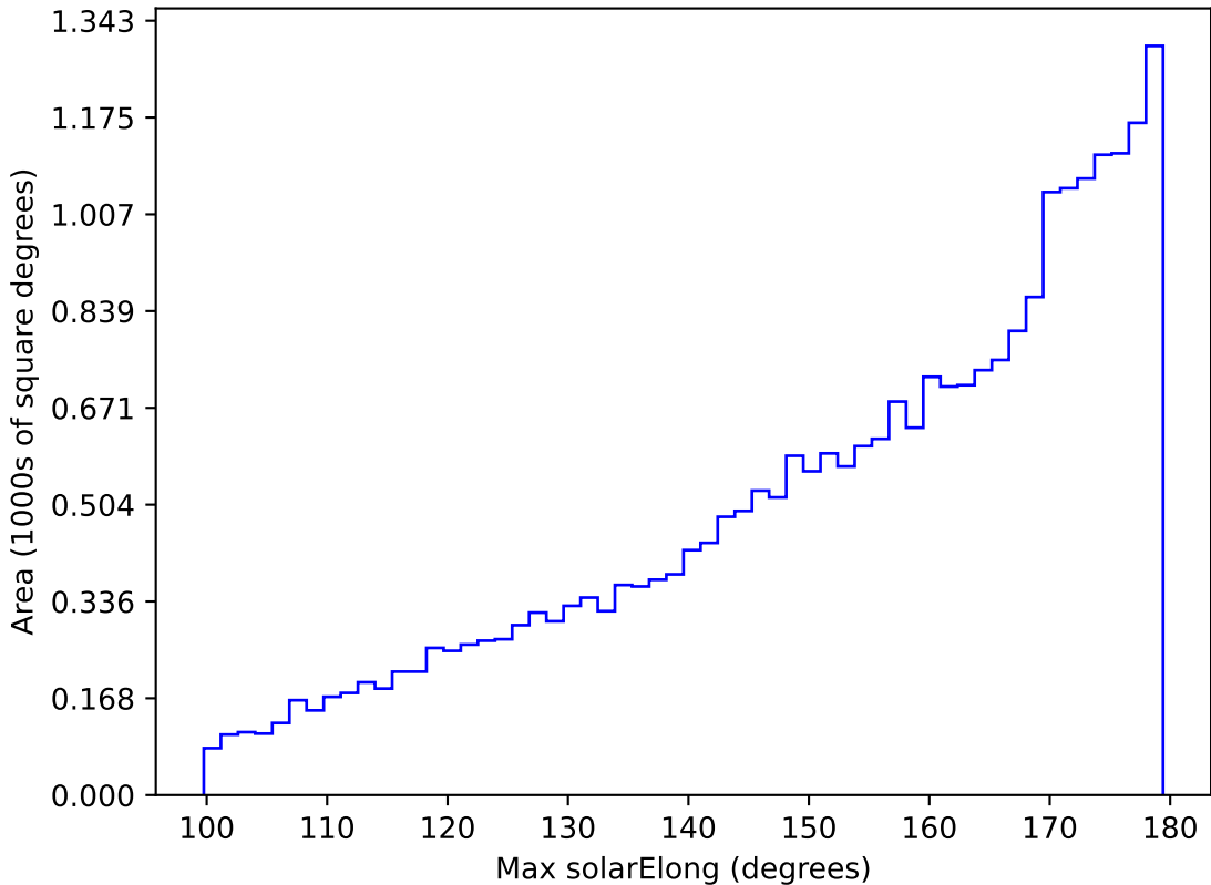
ddf_loaded_half_fl2_v3.4_10yrs All sky i band: Max solarElong
