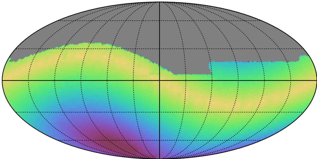
ddf_loaded_half_fl2_v3.4_10yrs All sky g band: Max solarElong
