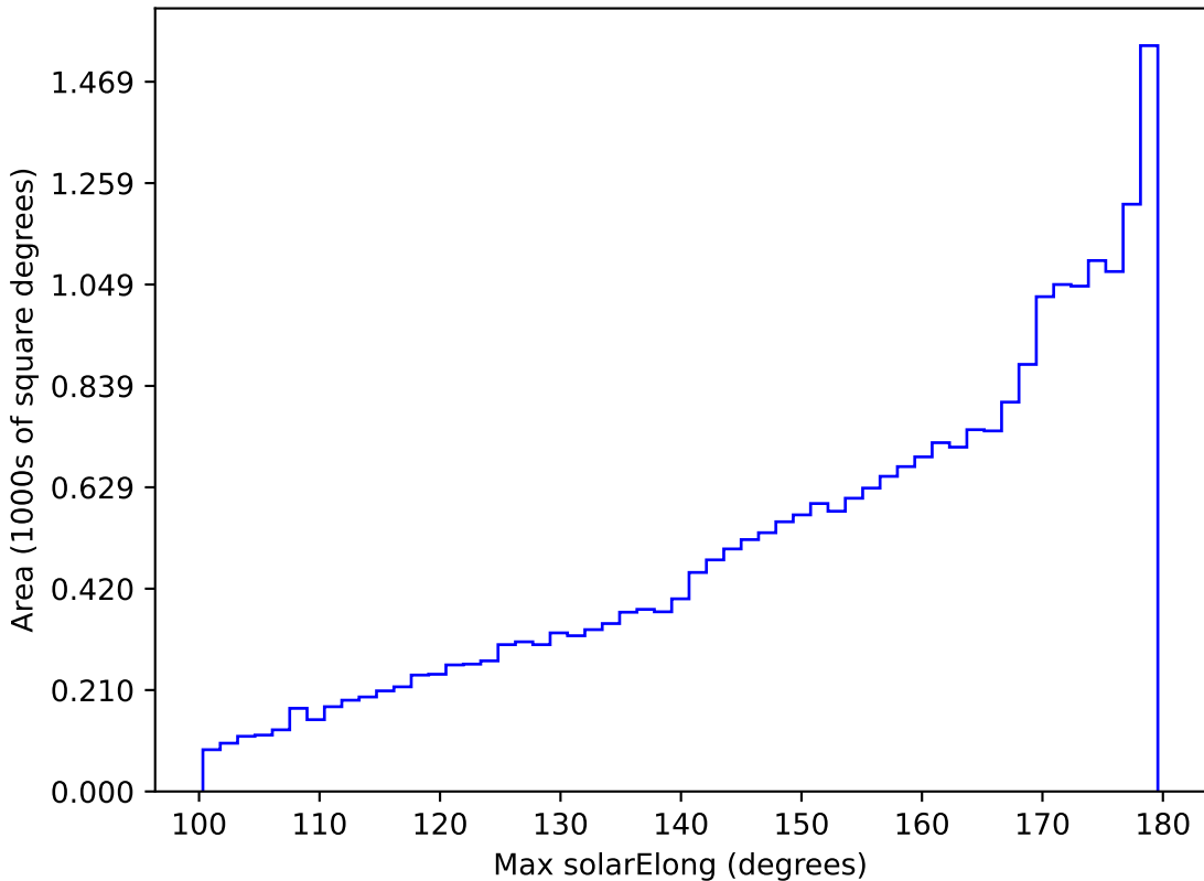
ddf_loaded_half_fl2_v3.4_10yrs All sky all bands: Max solarElong
