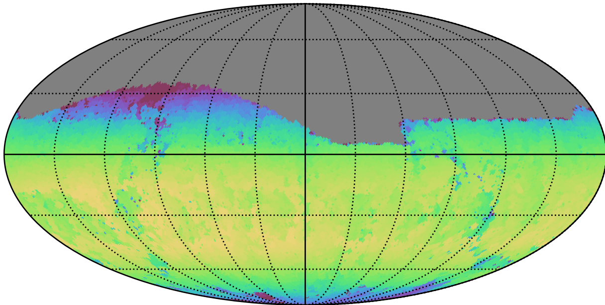
ddf_loaded_half_fl2_v3.4_10yrs Yr 1 z band: Max skyBrightness
