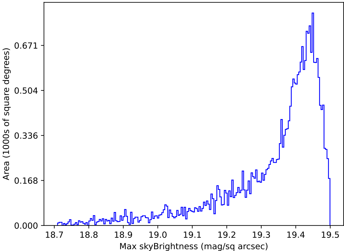
ddf_loaded_half_fl2_v3.4_10yrs Yr 1 z band: Max skyBrightness
