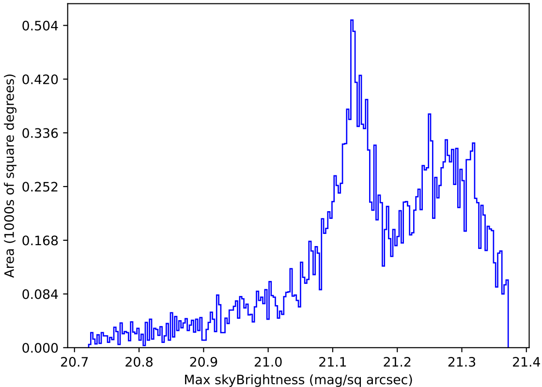
ddf_loaded_half_fl2_v3.4_10yrs Yr 1 r band: Max skyBrightness
