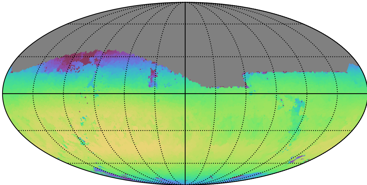
ddf_loaded_half_fl2_v3.4_10yrs Yr 1 i band: Max skyBrightness
