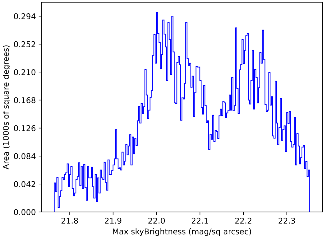
ddf_loaded_half_fl2_v3.4_10yrs Yr 1 g band: Max skyBrightness
