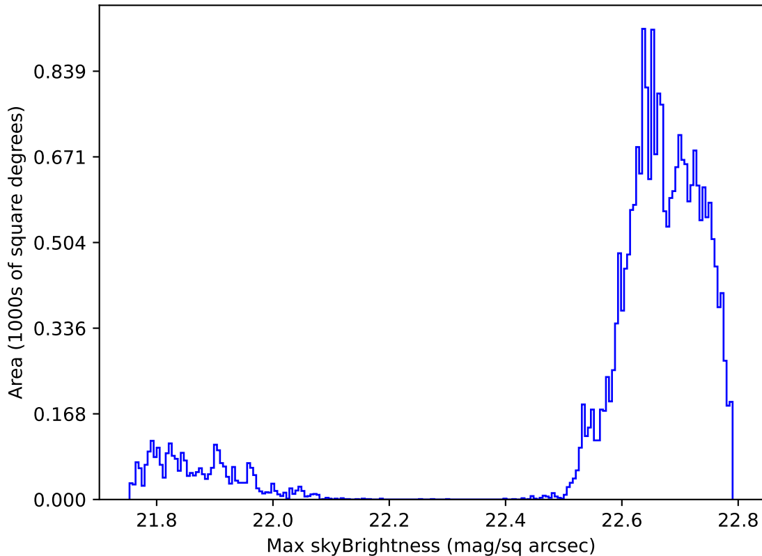
ddf_loaded_half_fl2_v3.4_10yrs Yr 1 all bands: Max skyBrightness
