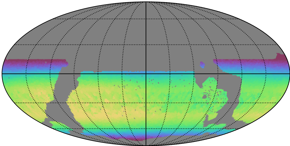
ddf_loaded_half_fl2_v3.4_10yrs WFD z band: Max skyBrightness
