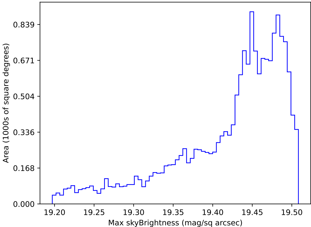
ddf_loaded_half_fl2_v3.4_10yrs WFD z band: Max skyBrightness
