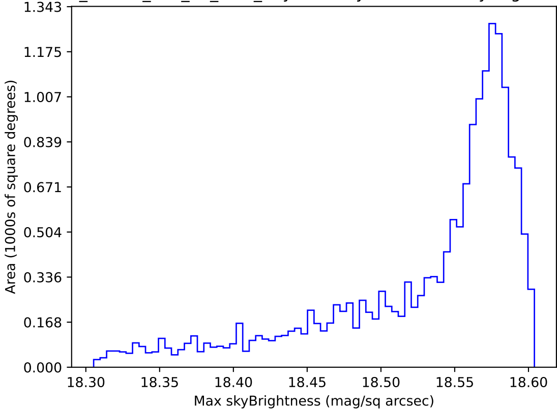
ddf_loaded_half_f12_v3.4_10yrs WFD y band: Max skyBrightness
