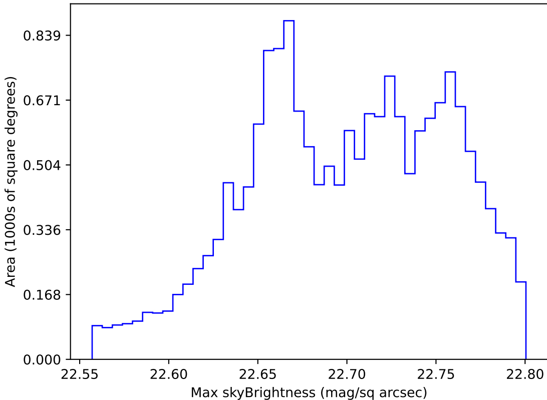
ddf_loaded_half_fl2_v3.4_10yrs WFD u band: Max skyBrightness
